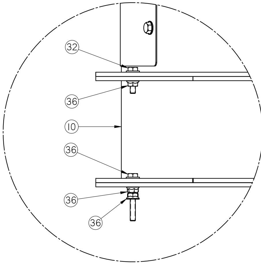
DETAIL B
