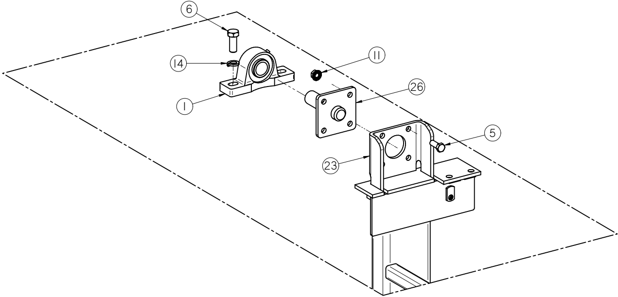
DETAIL A
