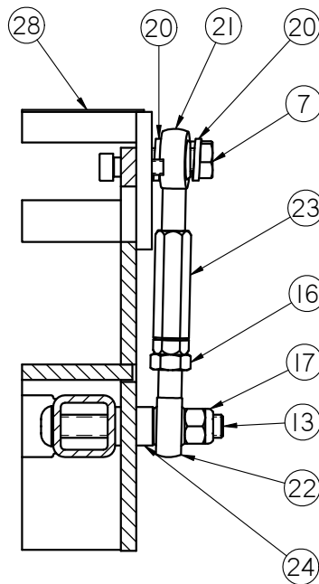
SECTION C-C
