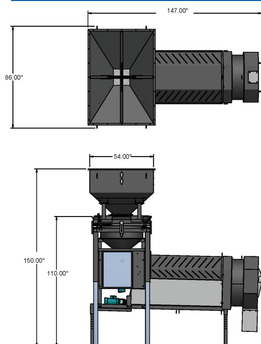
LIW STACKED OVER TREATER
