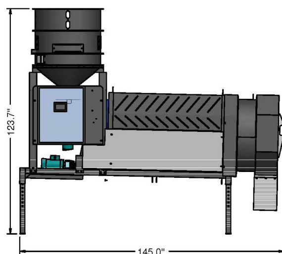
SEED WHEEL STACKED OVER TREATER
